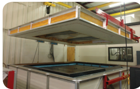
The Butler Guarded Hot Box tests actual in-place performance of insulation assemblies.
